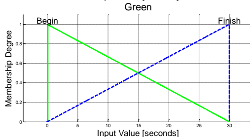
Figure 4 – Membership functions for the traffic light time, red and green respectively
